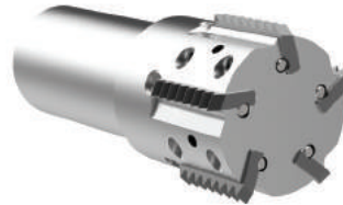
Weldon Pin Style AccuThread™ 856 Indexable
