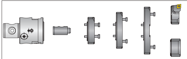
Imperial form 101 insert pictured | Kit No. 104065
